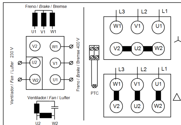
Figure 10: Motor connection schematics for MAC motors with 400 VAC brake (Not standard).
