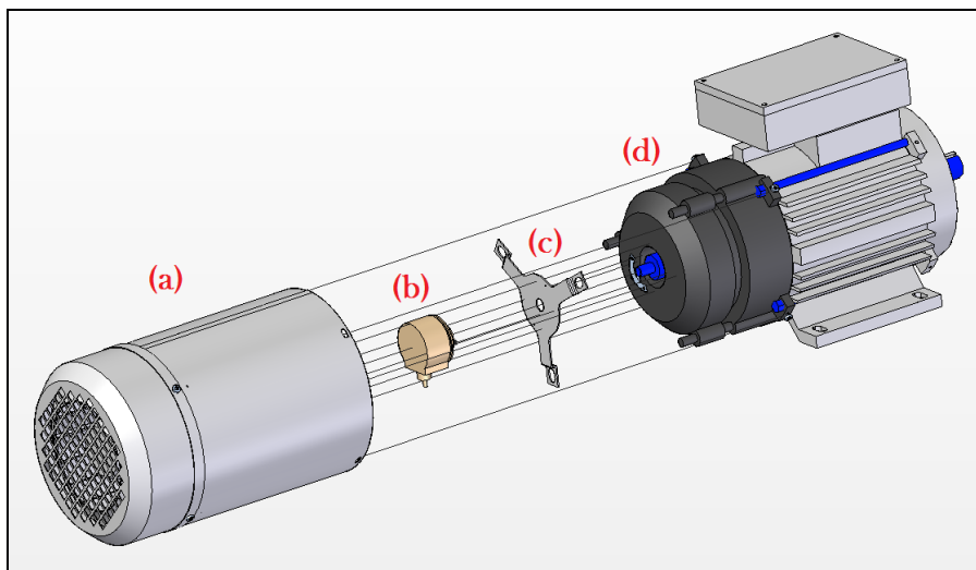
Figure 19: Replacing the brake on MAC R motors
