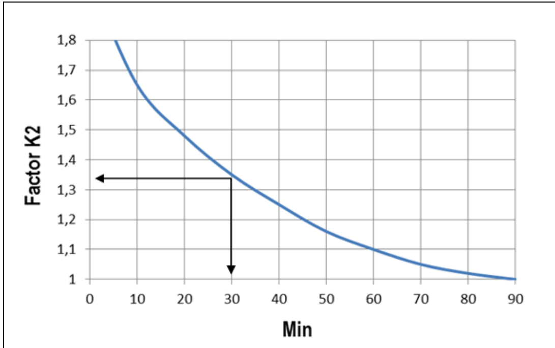
Figure 3: Derating factor for an S2-type service
