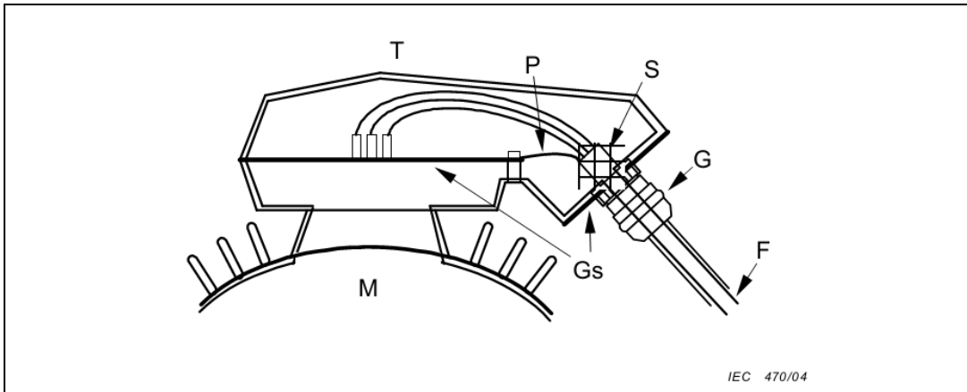
Figure 12: Recommended terminations
