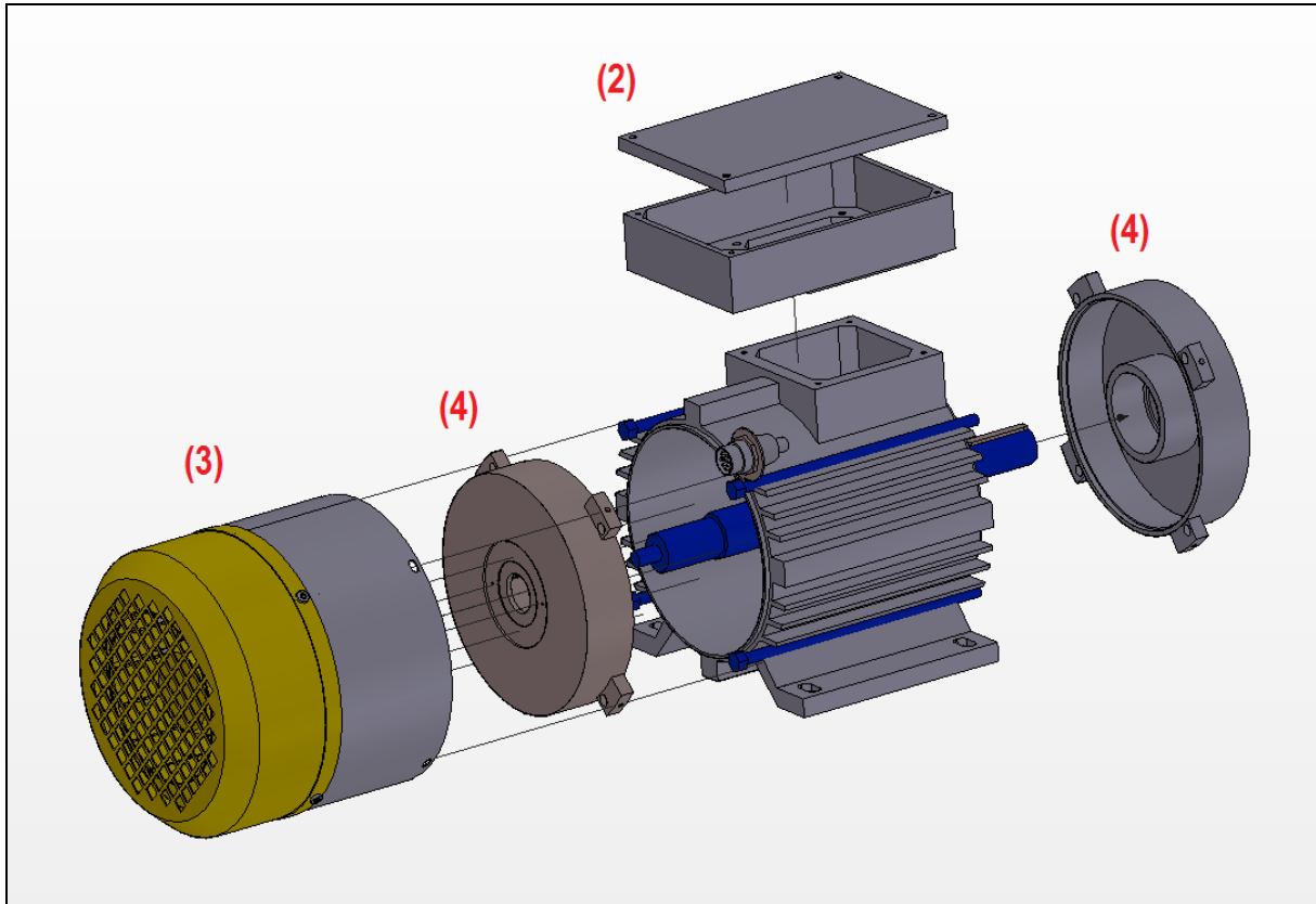
Figure 21: Spare subunits
