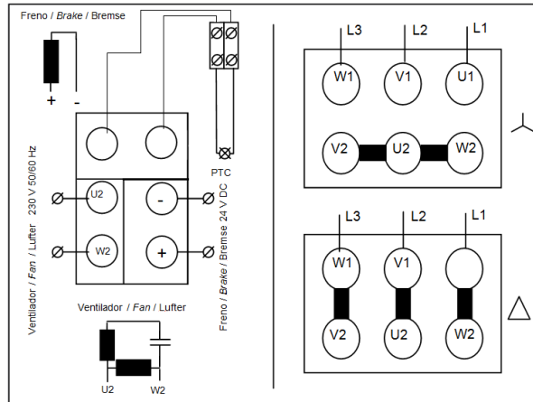
Figure 8: Motor connection schematics for MAC R 080, 090, 100, 112 and 132 motors with 24 VDC brake
