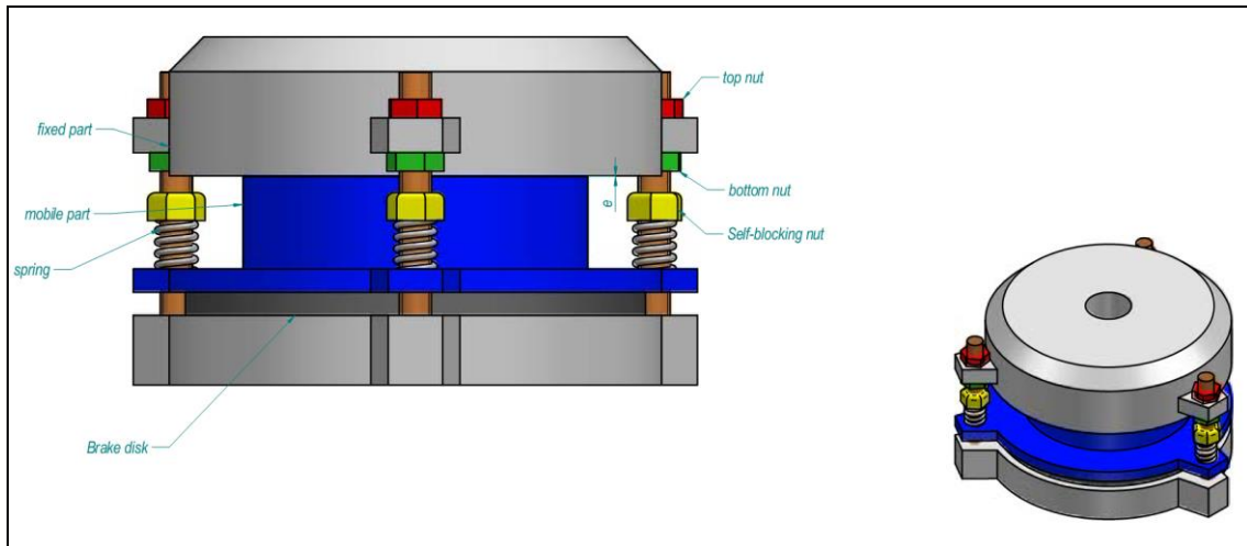
Figure 18: Brake adjustment
