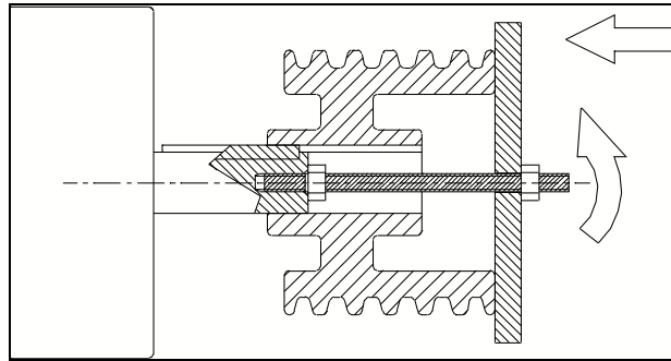
Figure 7: Fitting the coupling
