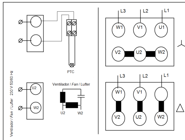
Figure 9: Motor connection schematics for MAC R 160 motors
