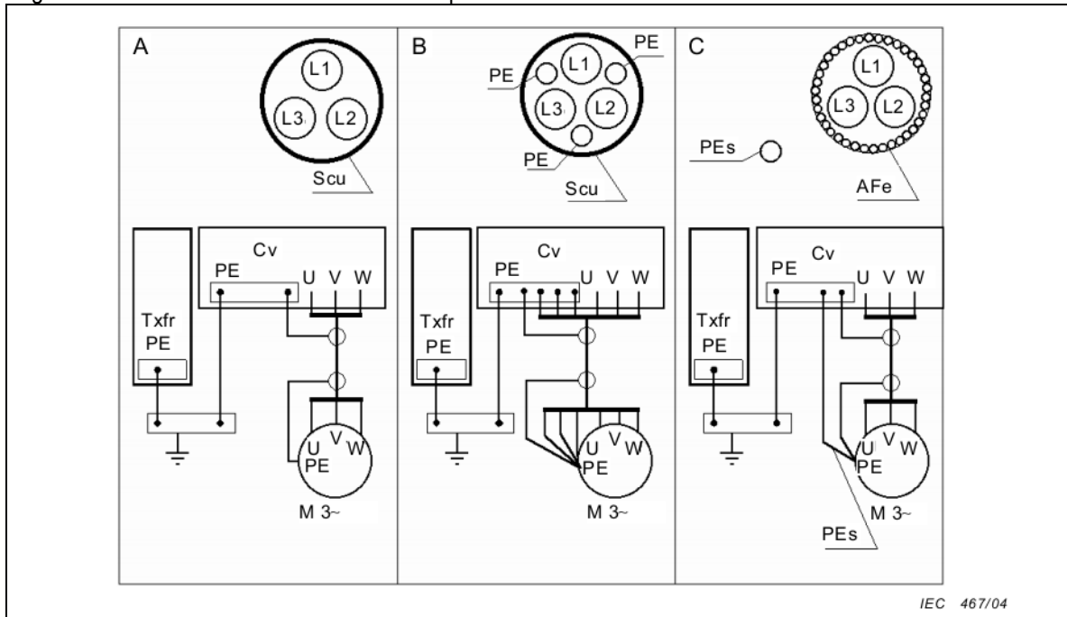
Figure 11: Recommended power cables and connections
