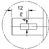
Detail A 2:1 Groove for woodruff key 4x 5 DIN 6888 Series A
